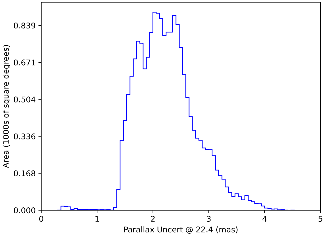
too_5_1v3.4_10yrs WFD: Parallax Uncert @ 22.4
