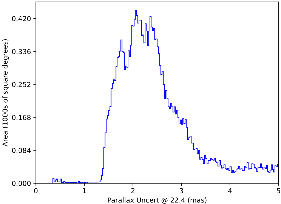
too_5_1v3.4_10yrs All sky: Parallax Uncert @ 22.4
