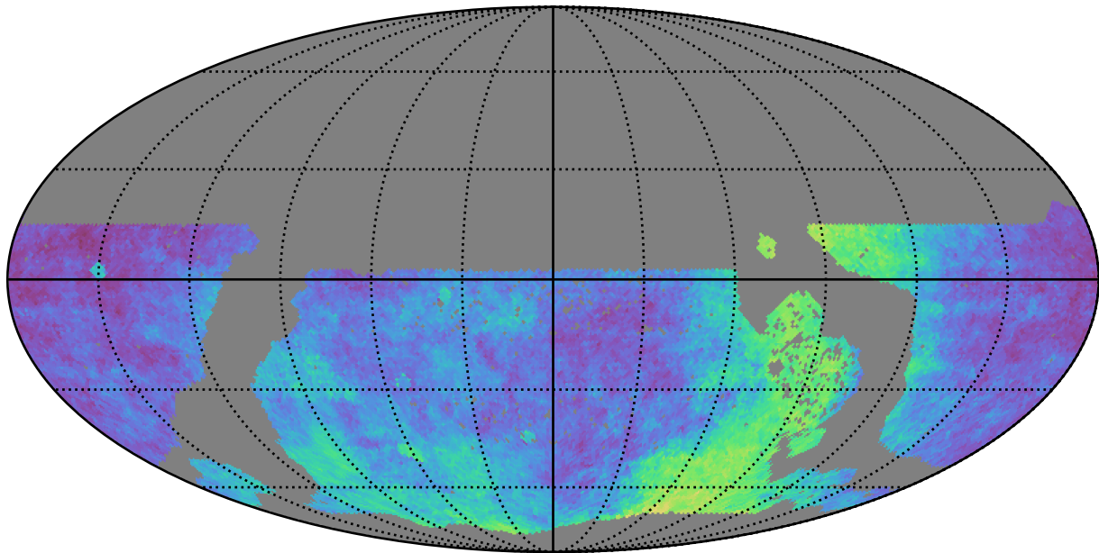
too_5_1v3.4_10yrs WFD: Parallax Coverage @ 24.0
