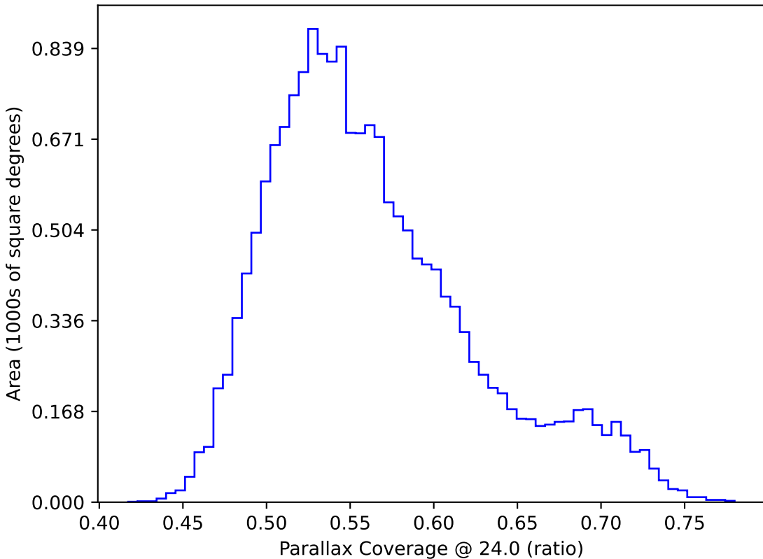
too_5_1v3.4_10yrs WFD: Parallax Coverage @ 24.0
