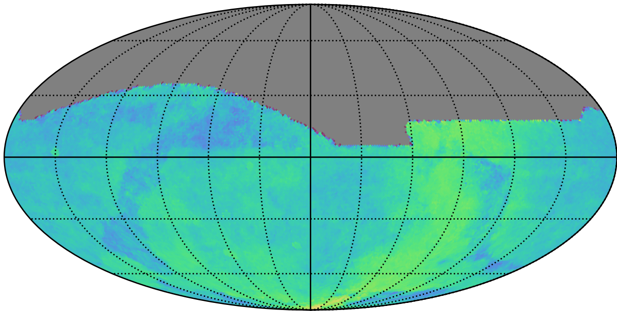
too_5_1v3.4_10yrs All sky: Parallax Coverage @ 24.0
