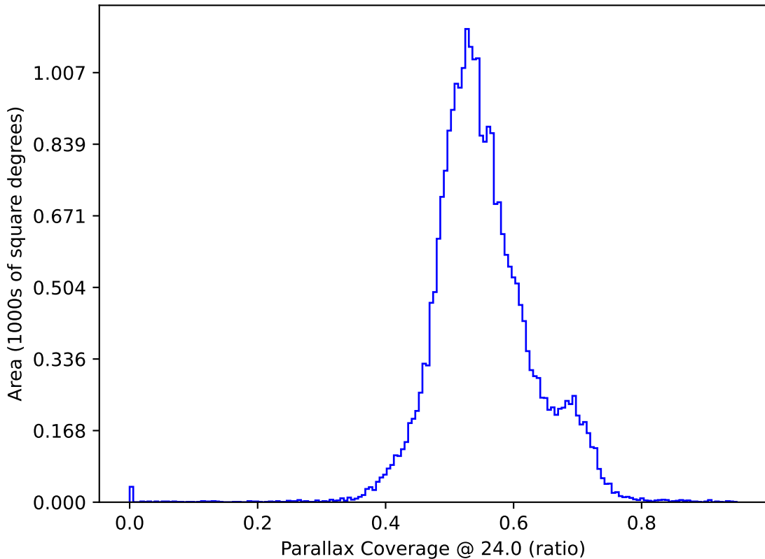
too_5_1v3.4_10yrs All sky: Parallax Coverage @ 24.0
