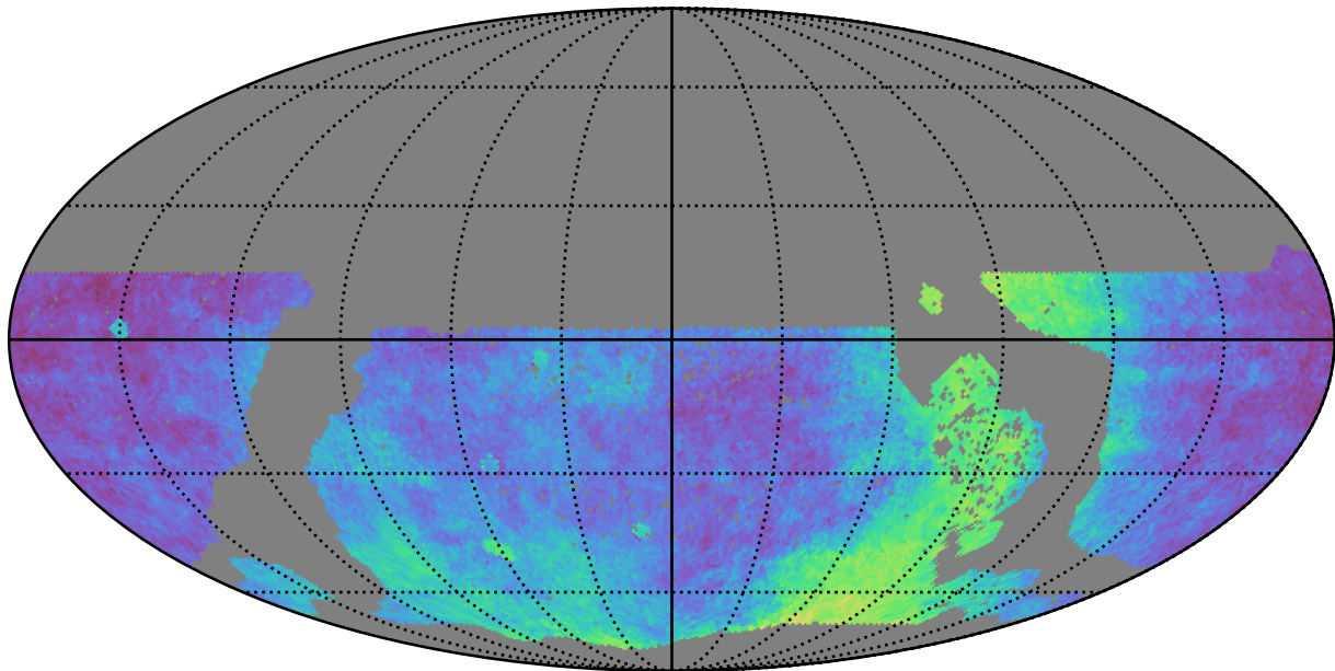
too_5_1v3.4_10yrs WFD: Parallax Coverage @ 22.4
