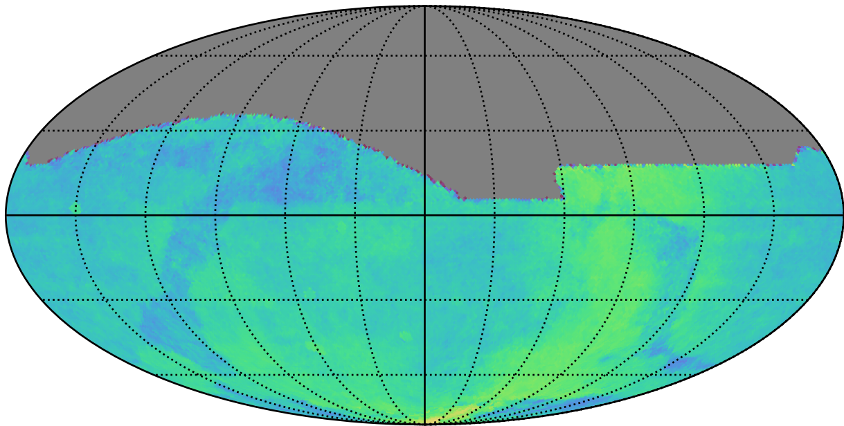
too_5_1v3.4_10yrs All sky: Parallax Coverage @ 22.4
