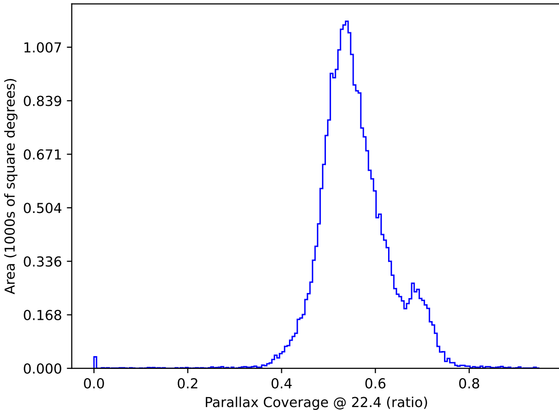
too_5_1v3.4_10yrs All sky: Parallax Coverage @ 22.4
