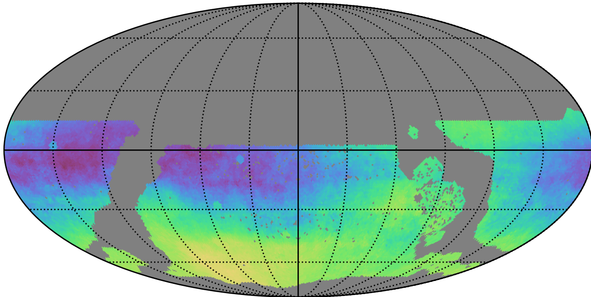
too_5_1v3.4_10yrs WFD: Parallax-DCR degeneracy @ 24.0
