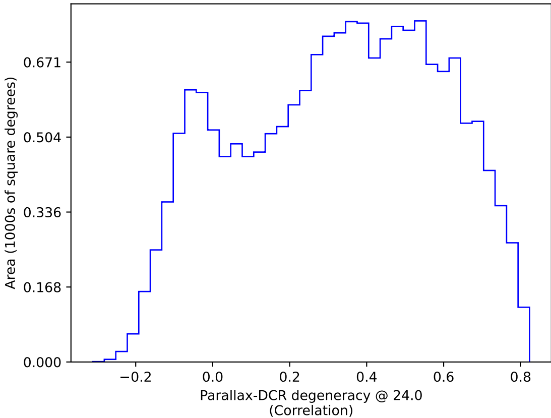
too_5_1v3.4_10yrs WFD: Parallax-DCR degeneracy @ 24.0
