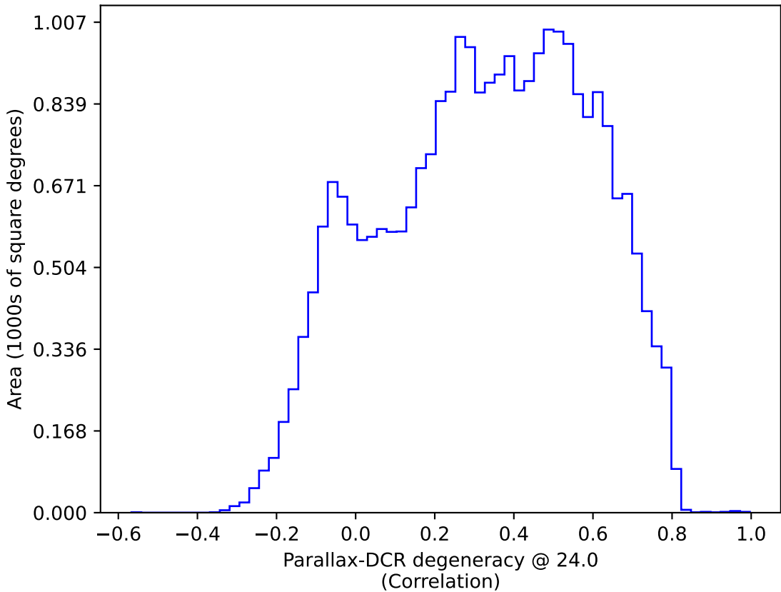
too_5_1v3.4_10yrs All sky: Parallax-DCR degeneracy @ 24.0
