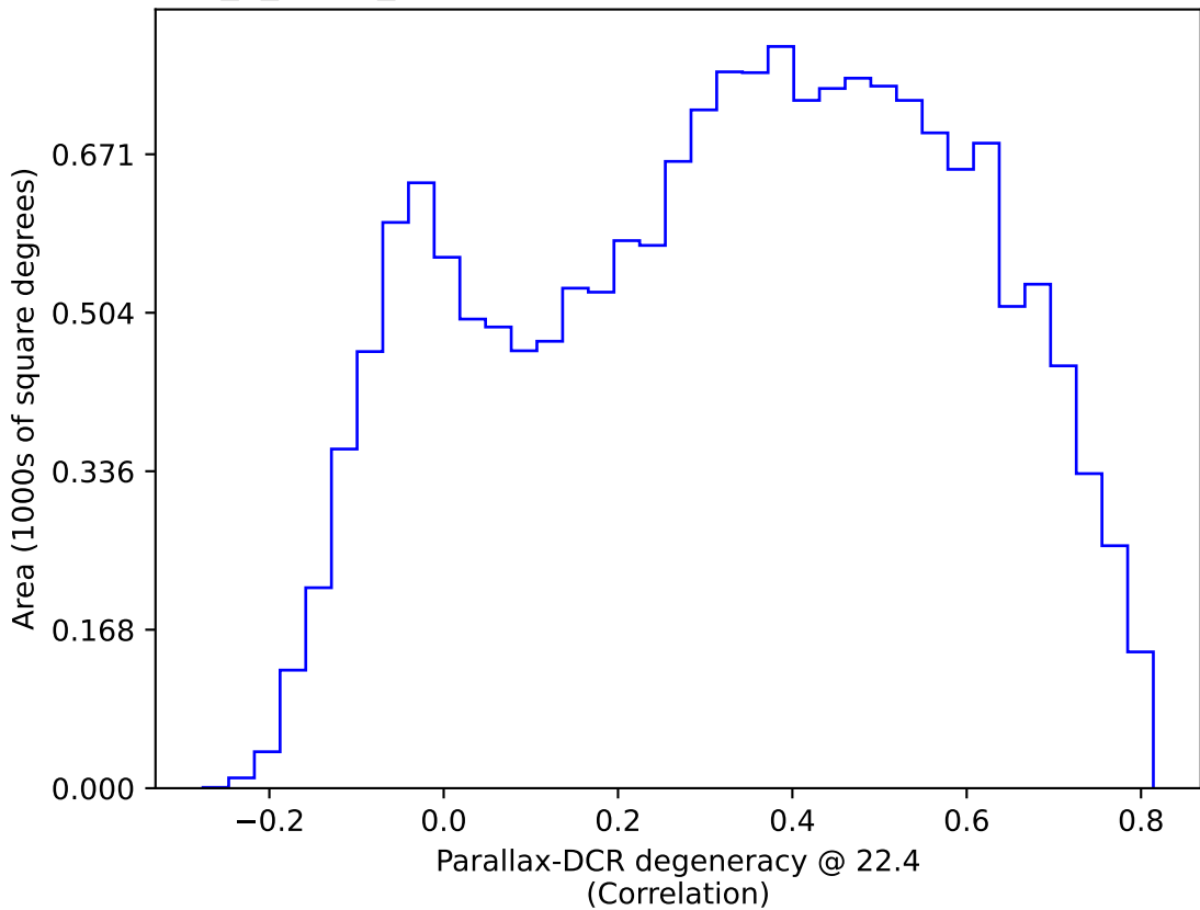
too_5_1v3.4_10yrs WFD: Parallax-DCR degeneracy @ 22.4
