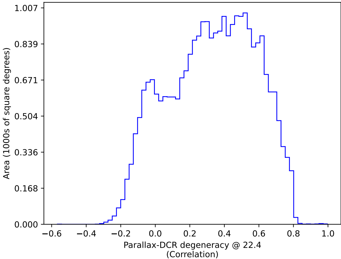
too_5_1v3.4_10yrs All sky: Parallax-DCR degeneracy @ 22.4
