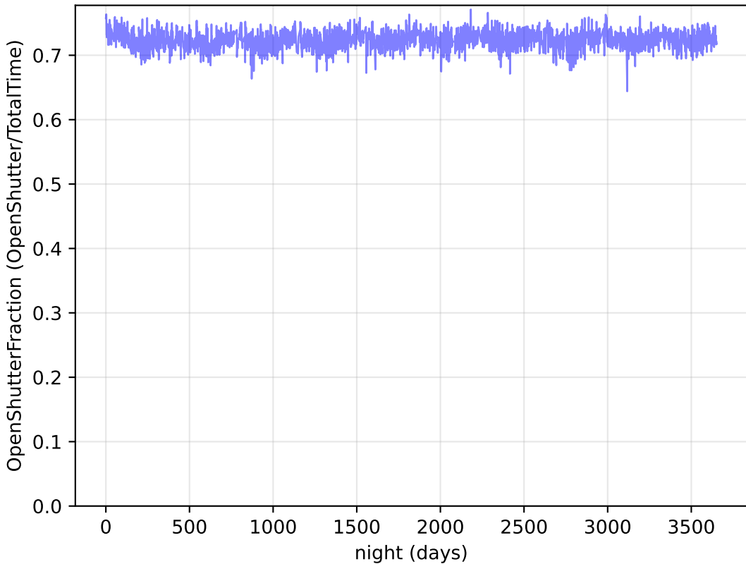
too_5_1v3.4_10yrs Per night: OpenShutterFraction
