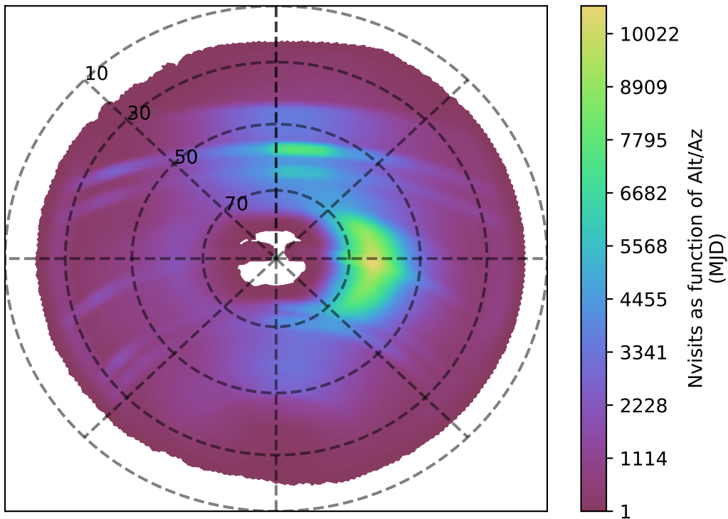
too_5_1v3.4_10yrs all bands: Nvisits as function of Alt/Az
