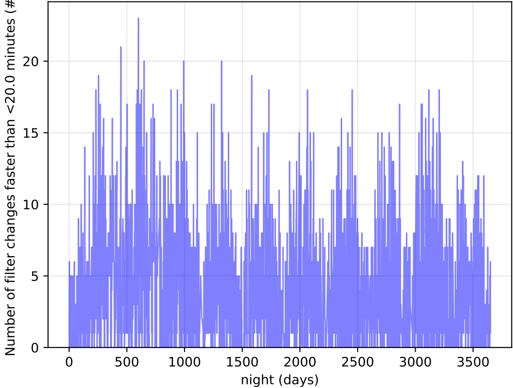
too_5_1v3.4_10yrs Per Night: Number of filter changes faster than <20.0 minutes
