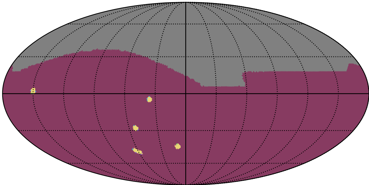
too_5_1v3.4_10yrs All sky: NumberOfQuickRevisits
