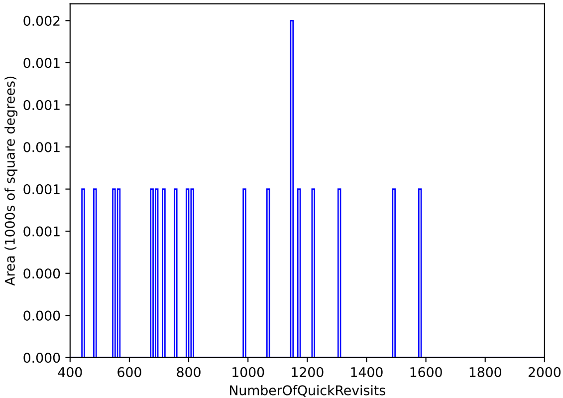
too_5_1v3.4_10yrs All sky: NumberOfQuickRevisits
