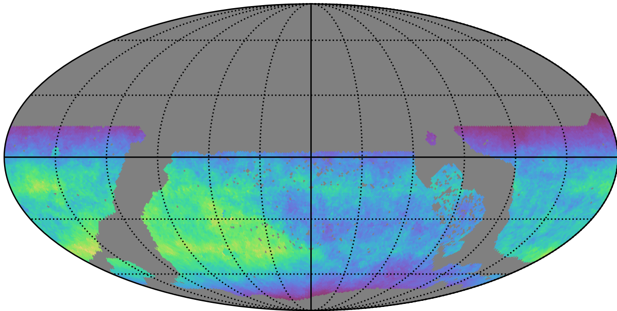
too_5_1v3.4_10yrs WFD z band: Normalized Teff
