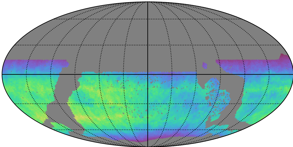
too_5_1v3.4_10yrs WFD y band: Normalized Teff
