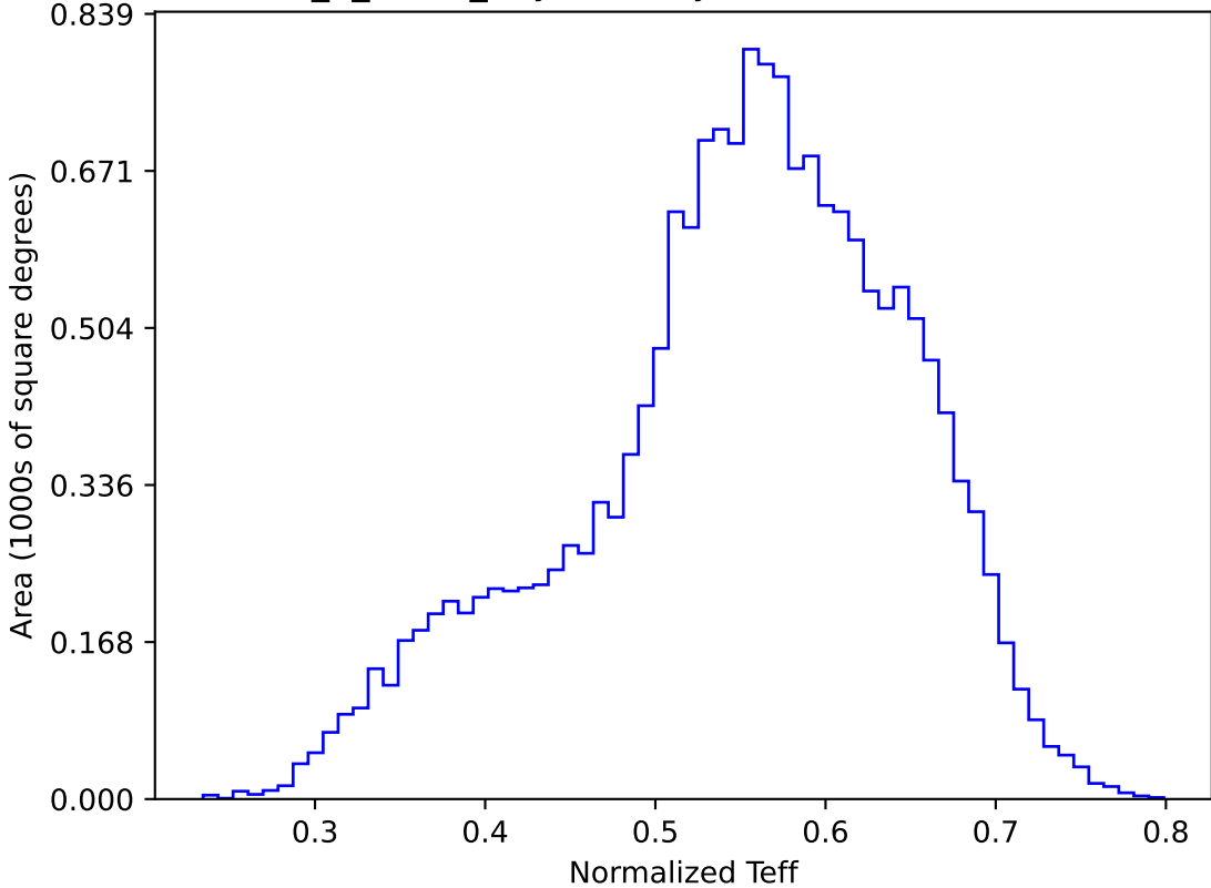
too_5_1v3.4_10yrs WFD y band: Normalized Teff
