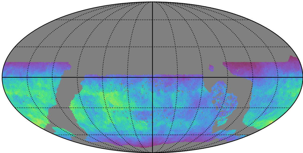
too_5_1v3.4_10yrs WFD u band: Normalized Teff
