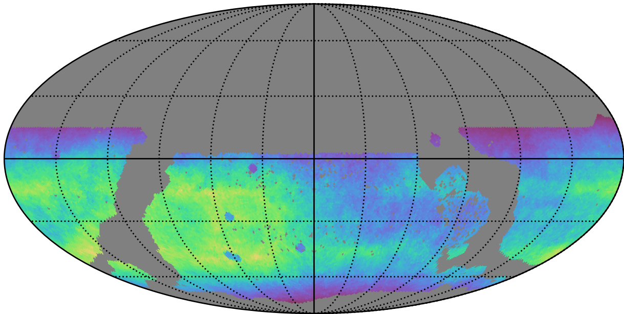
too_5_1v3.4_10yrs WFD r band: Normalized Teff
