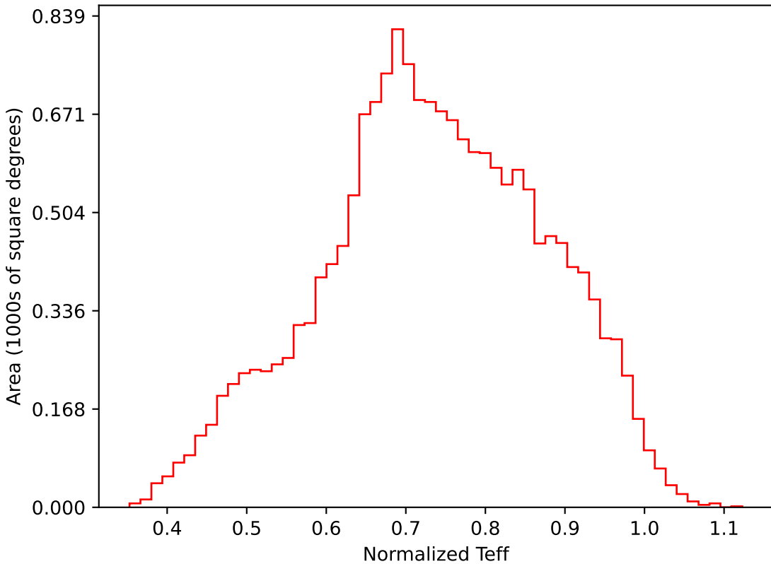
too_5_1v3.4_10yrs WFD i band: Normalized Teff
