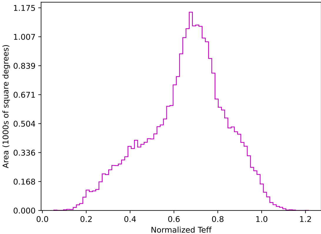
too_5_1v3.4_10yrs All sky z band: Normalized Teff
