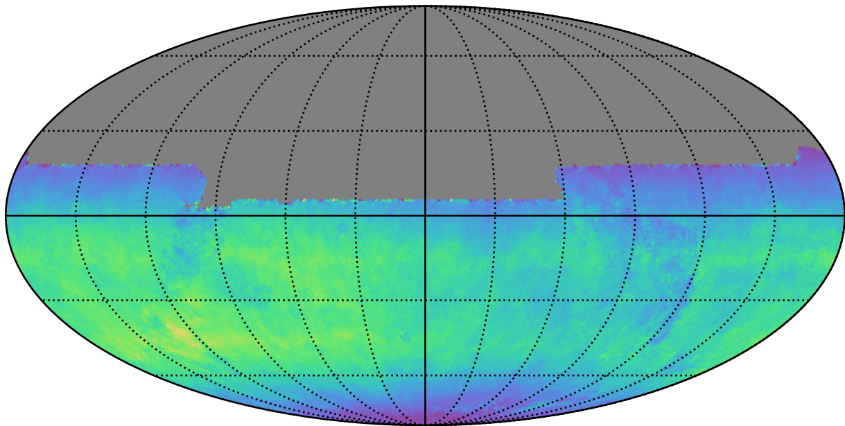
too_5_1v3.4_10yrs All sky y band: Normalized Teff
