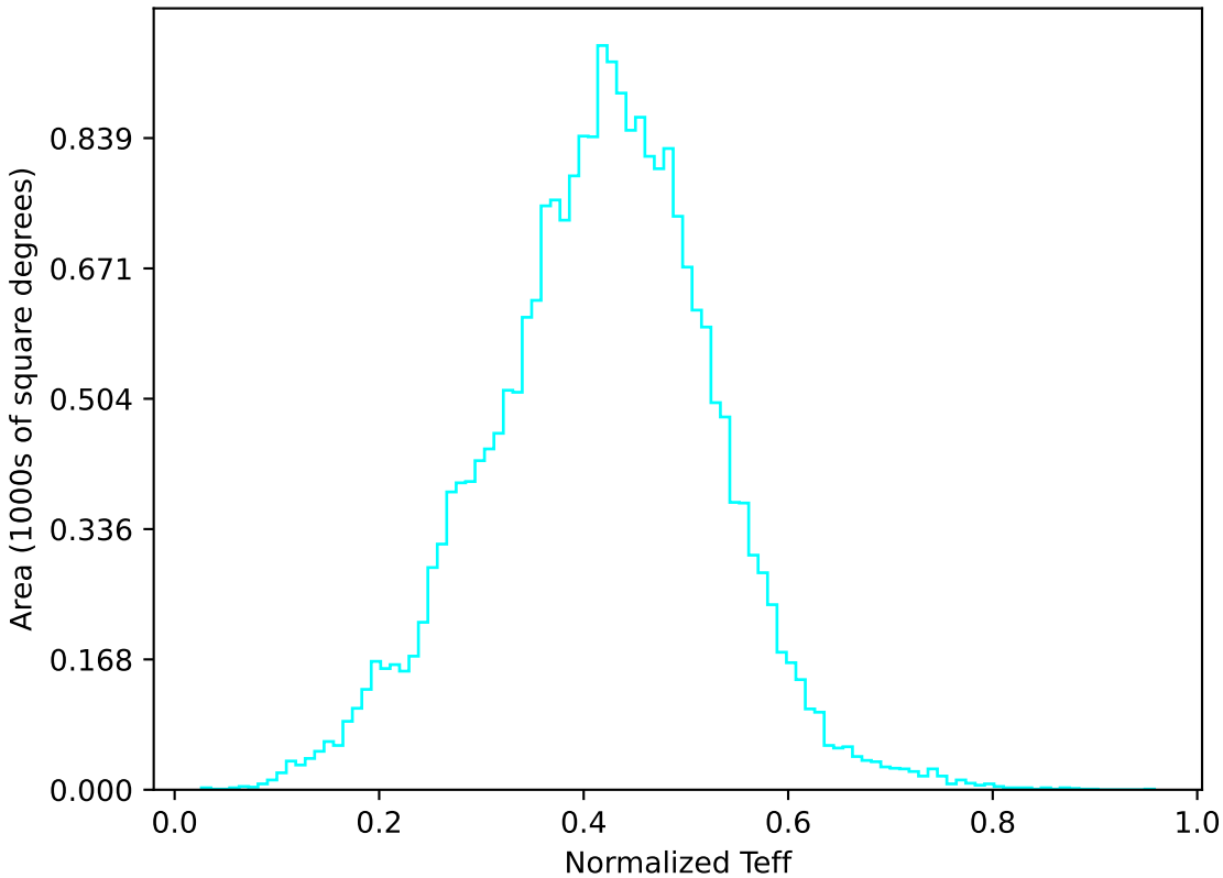
too_5_1v3.4_10yrs All sky u band: Normalized Teff
