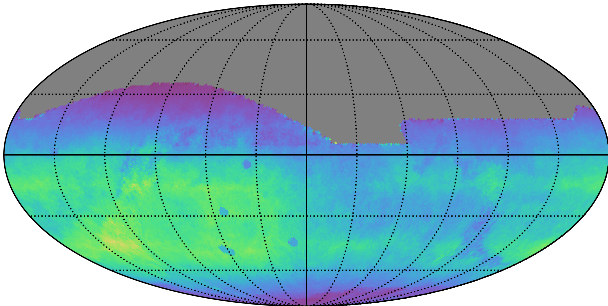
too_5_1v3.4_10yrs All sky r band: Normalized Teff
