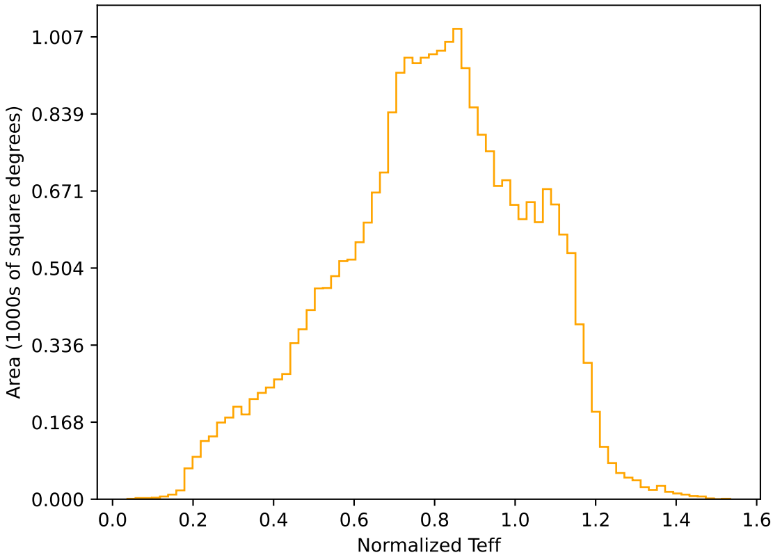
too_5_1v3.4_10yrs All sky r band: Normalized Teff
