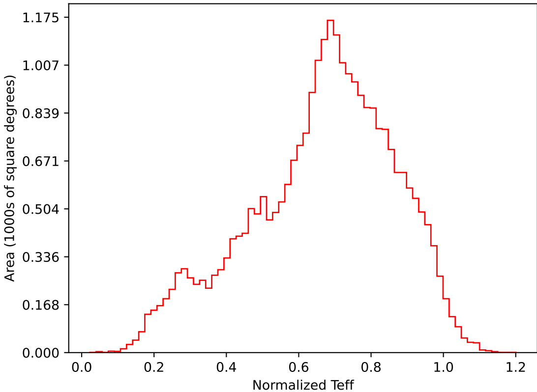
too_5_1v3.4_10yrs All sky i band: Normalized Teff
