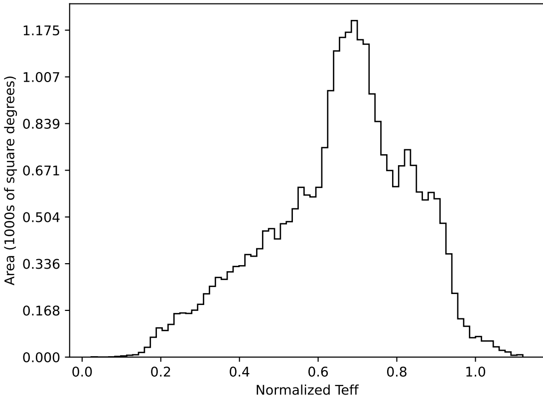
too_5_1v3.4_10yrs All sky all bands: Normalized Teff
