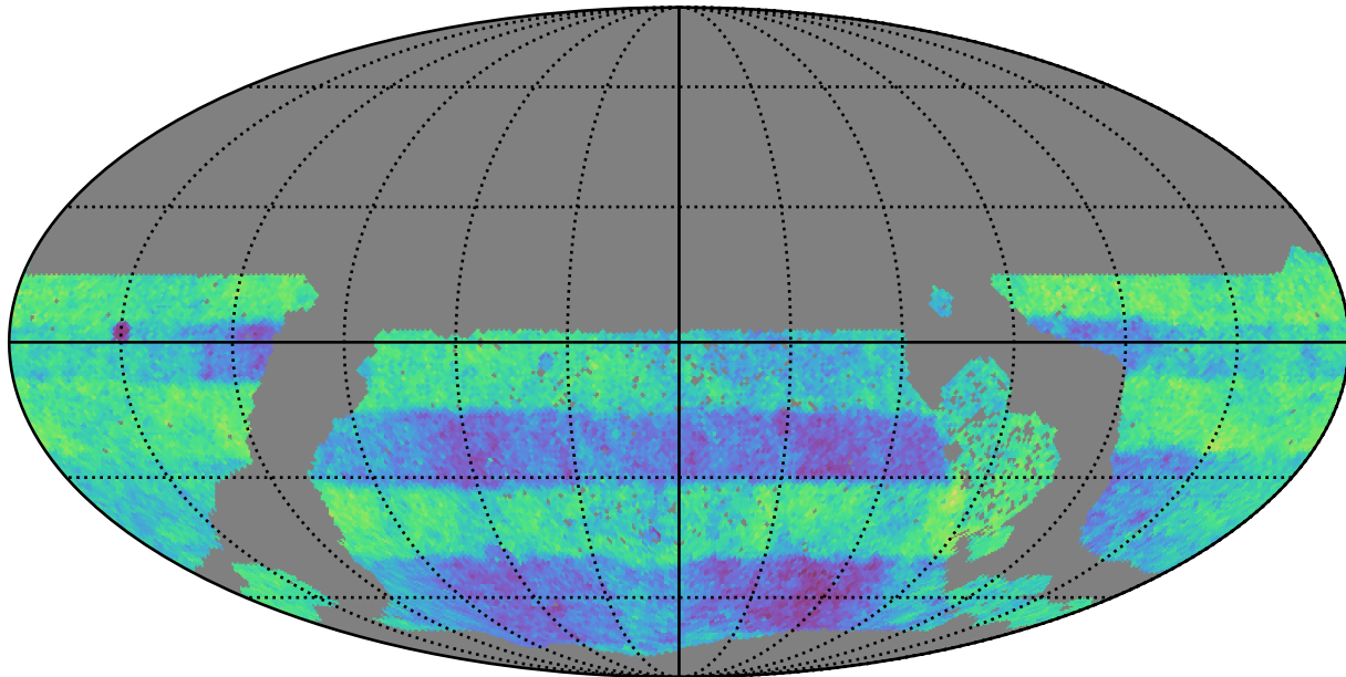
too_5_1v3.4_10yrs WFD: Normalized Proper Motion Uncert @ 24.0
