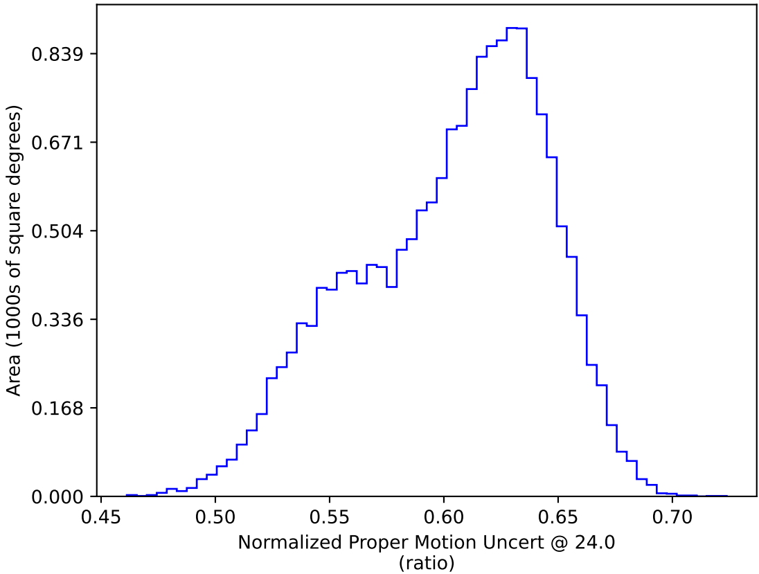
too_5_1v3.4_10yrs WFD: Normalized Proper Motion Uncert @ 24.0
