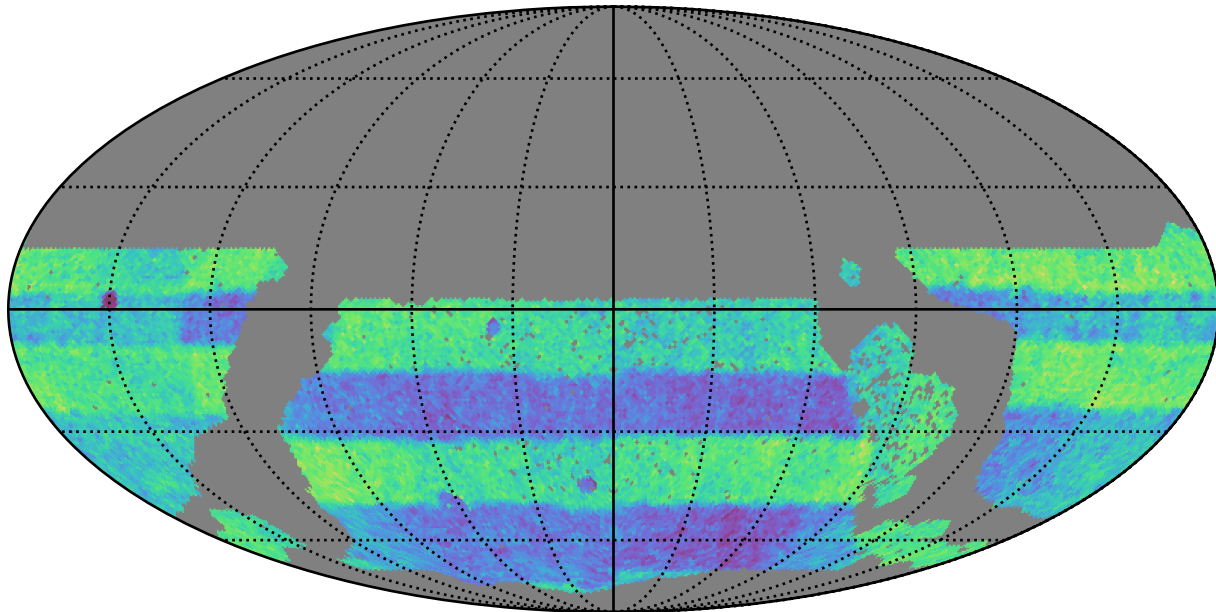
too_5_1v3.4_10yrs WFD: Normalized Proper Motion Uncert @ 20.5
