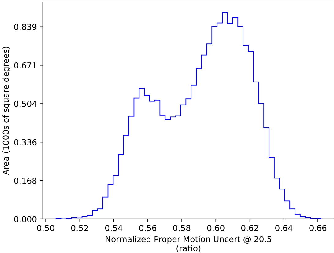
too_5_1v3.4_10yrs WFD: Normalized Proper Motion Uncert @ 20.5
