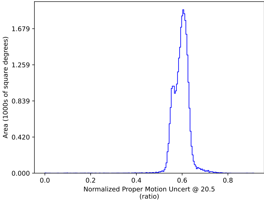
too_5_1v3.4_10yrs All sky: Normalized Proper Motion Uncert @ 20.5
