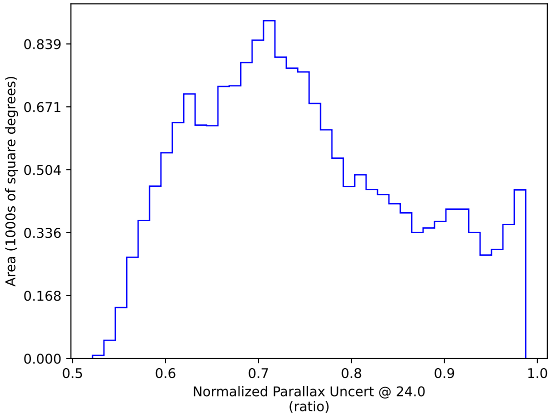
too_5_1v3.4_10yrs WFD: Normalized Parallax Uncert @ 24.0
