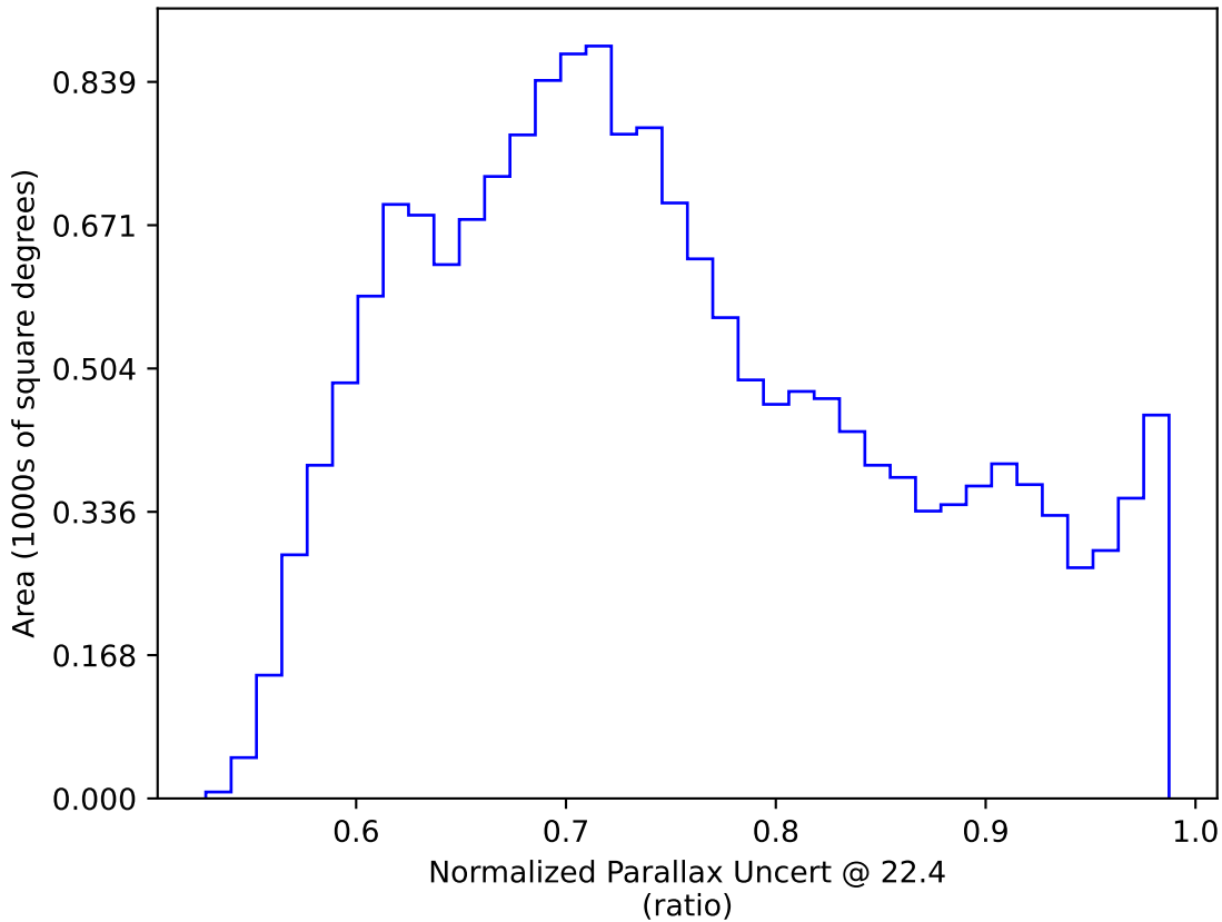
too_5_1v3.4_10yrs WFD: Normalized Parallax Uncert @ 22.4
