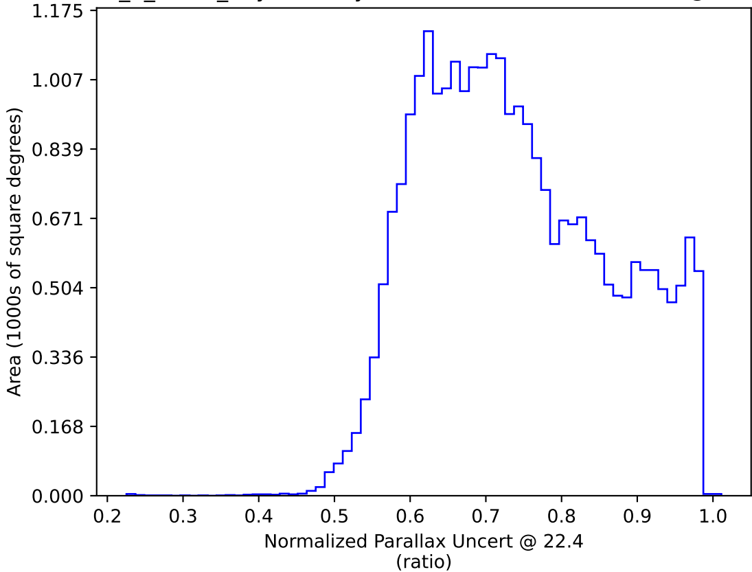
too_5_1v3.4_10yrs All sky: Normalized Parallax Uncert @ 22.4
