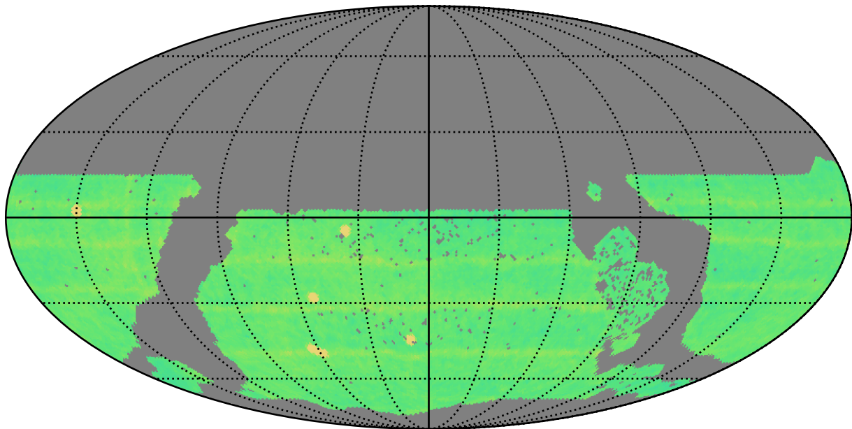
too_5_1v3.4_10yrs WFD all bands: N Unique Nights
