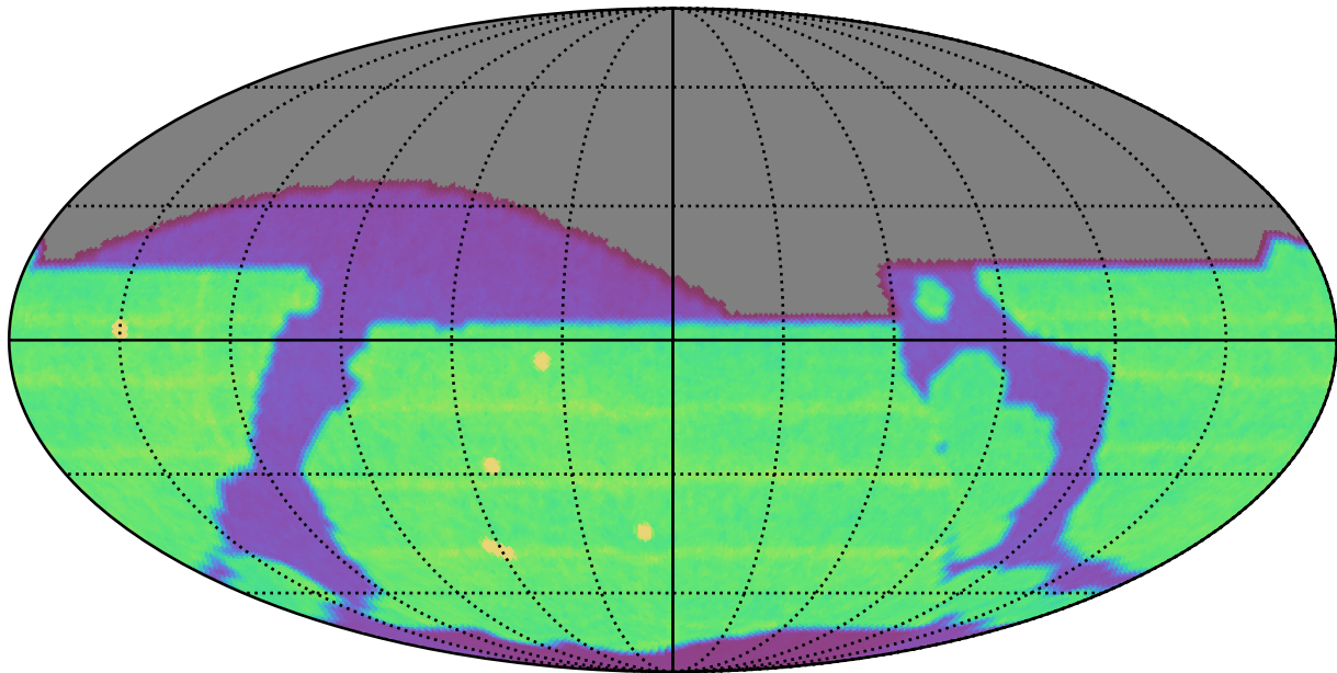
too_5_1v3.4_10yrs All sky all bands: N Unique Nights
