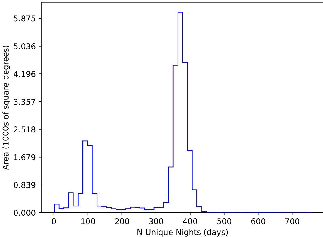
too_5_1v3.4_10yrs All sky all bands: N Unique Nights
