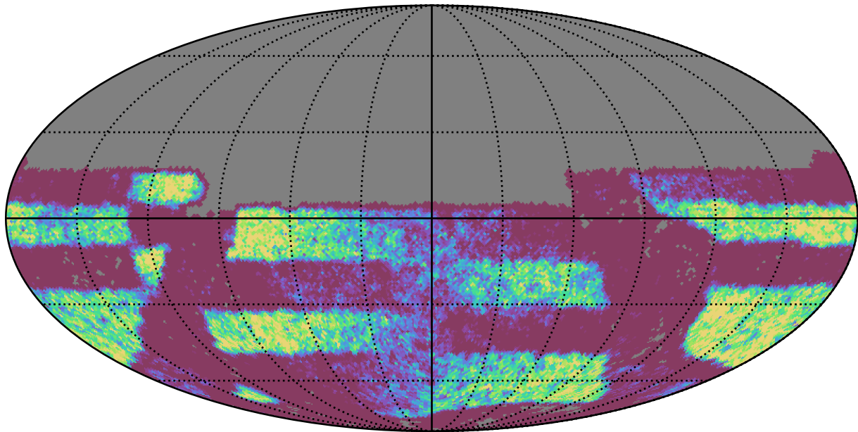
too_5_1v3.4_10yrs Yr 3-4 y band: NVisits
