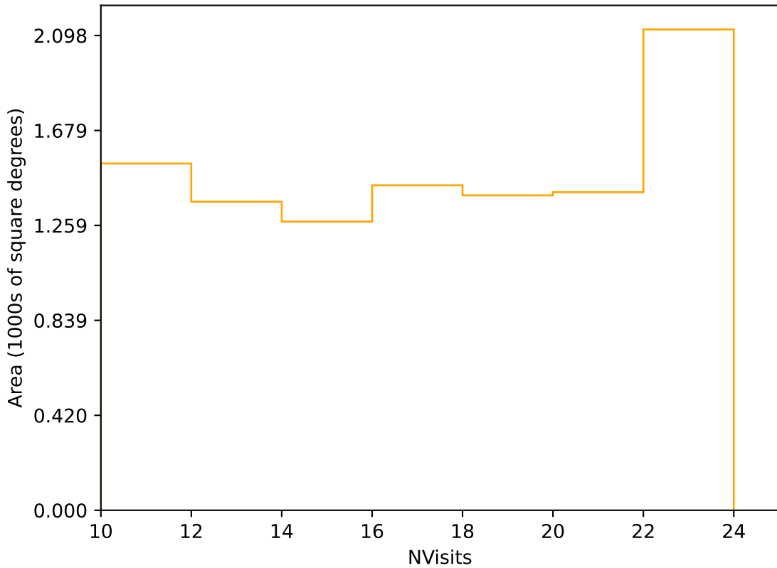
too_5_1v3.4_10yrs Yr 3-4 r band: NVisits
