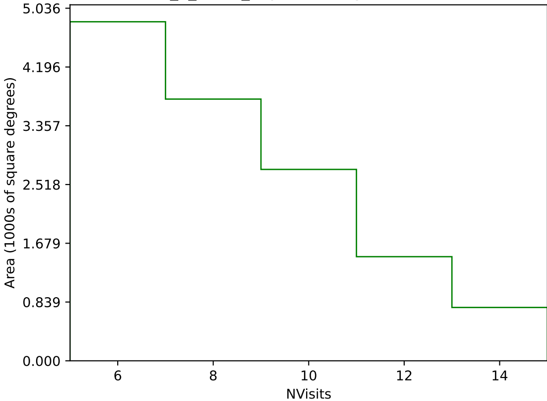
too_5_1v3.4_10yrs Yr 3-4 g band: NVisits
