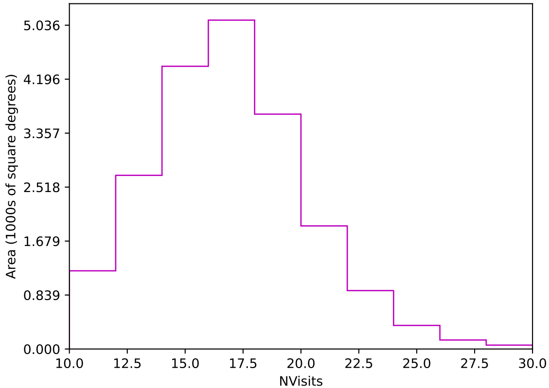
too_5_1v3.4_10yrs Yr 1 z band: NVisits
