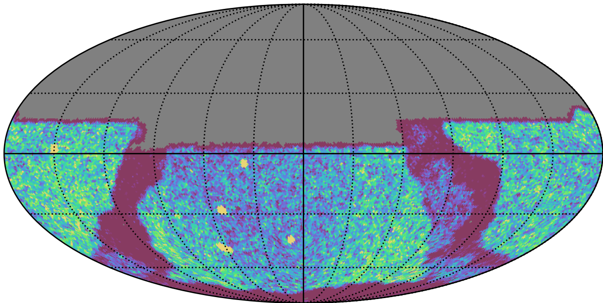
too_5_1v3.4_10yrs Yr 1 y band: NVisits
