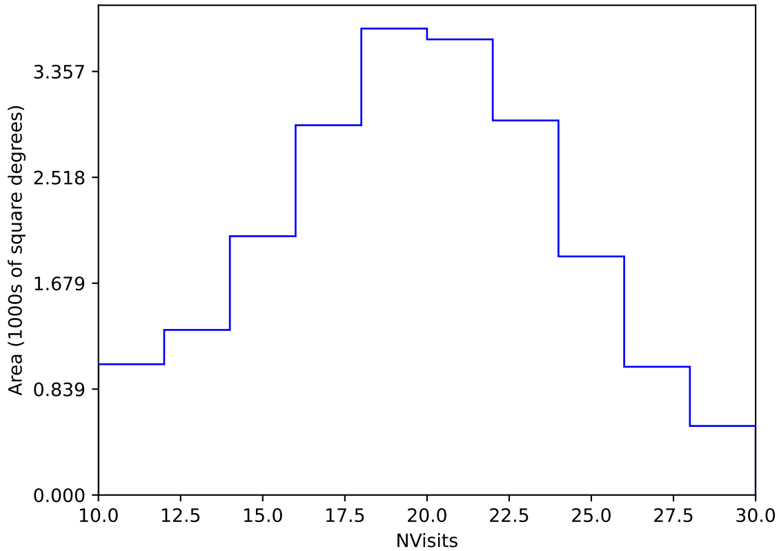
too_5_1v3.4_10yrs Yr 1 y band: NVisits
