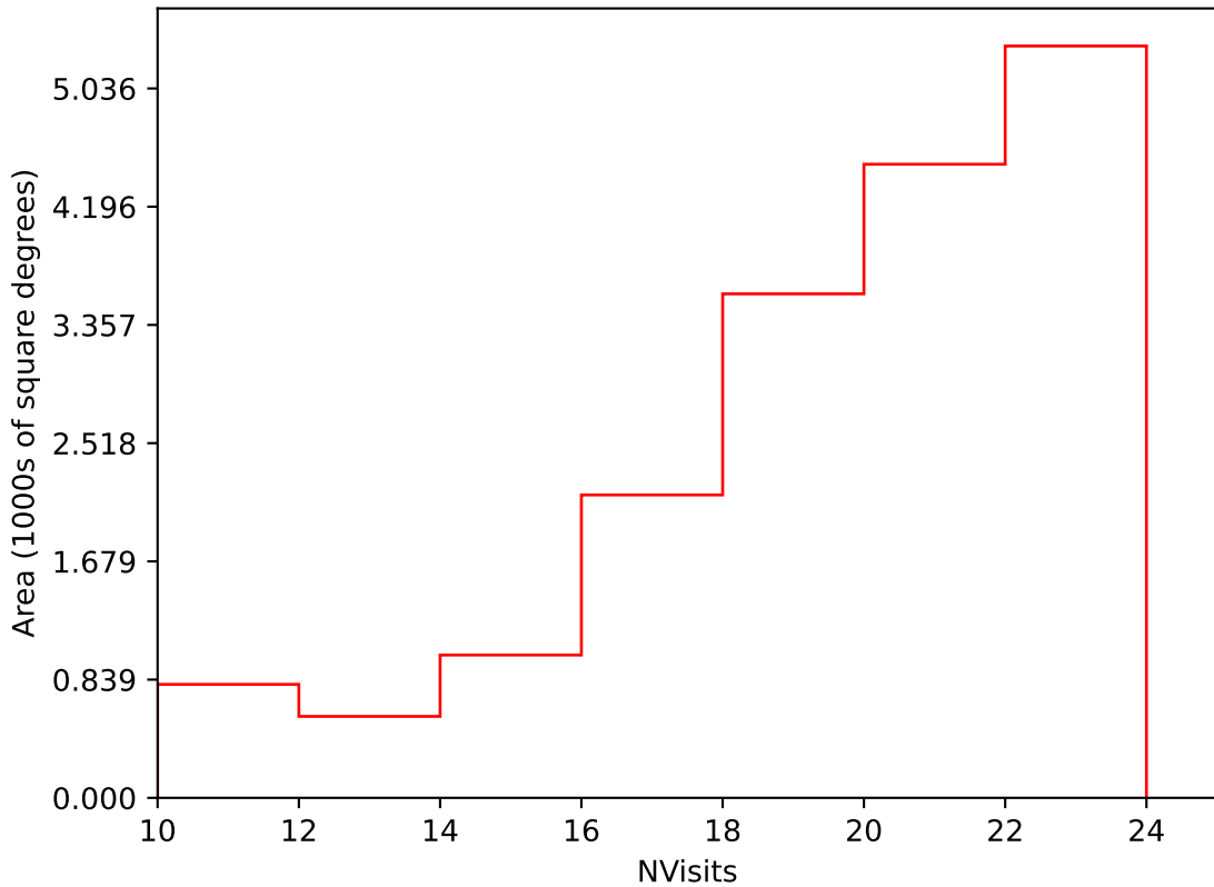
too_5_1v3.4_10yrs Yr 1 i band: NVisits
